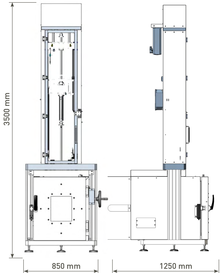
Dimensions with climatic chamber
