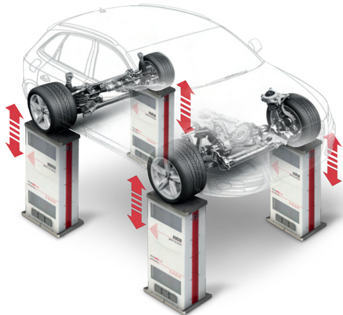
Damper Test System HUD020 with 4 synchronized actuators
